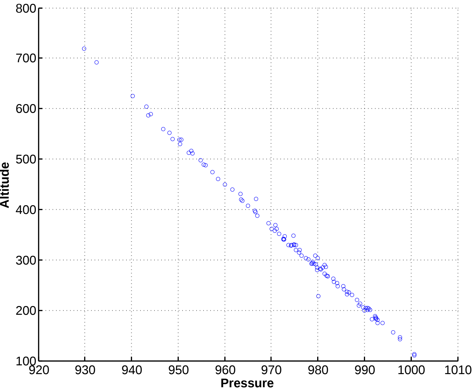
Pressure/Altitude test
