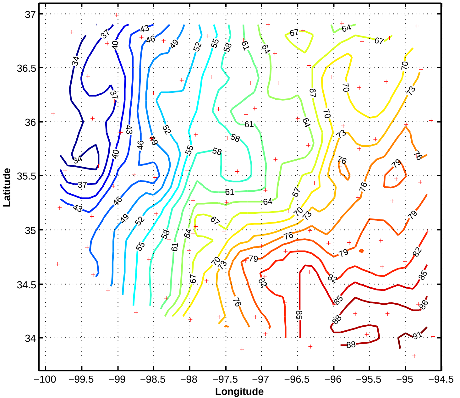
6/11/97 1800z Mesonet Pressures (units .1mb above 970mb)
