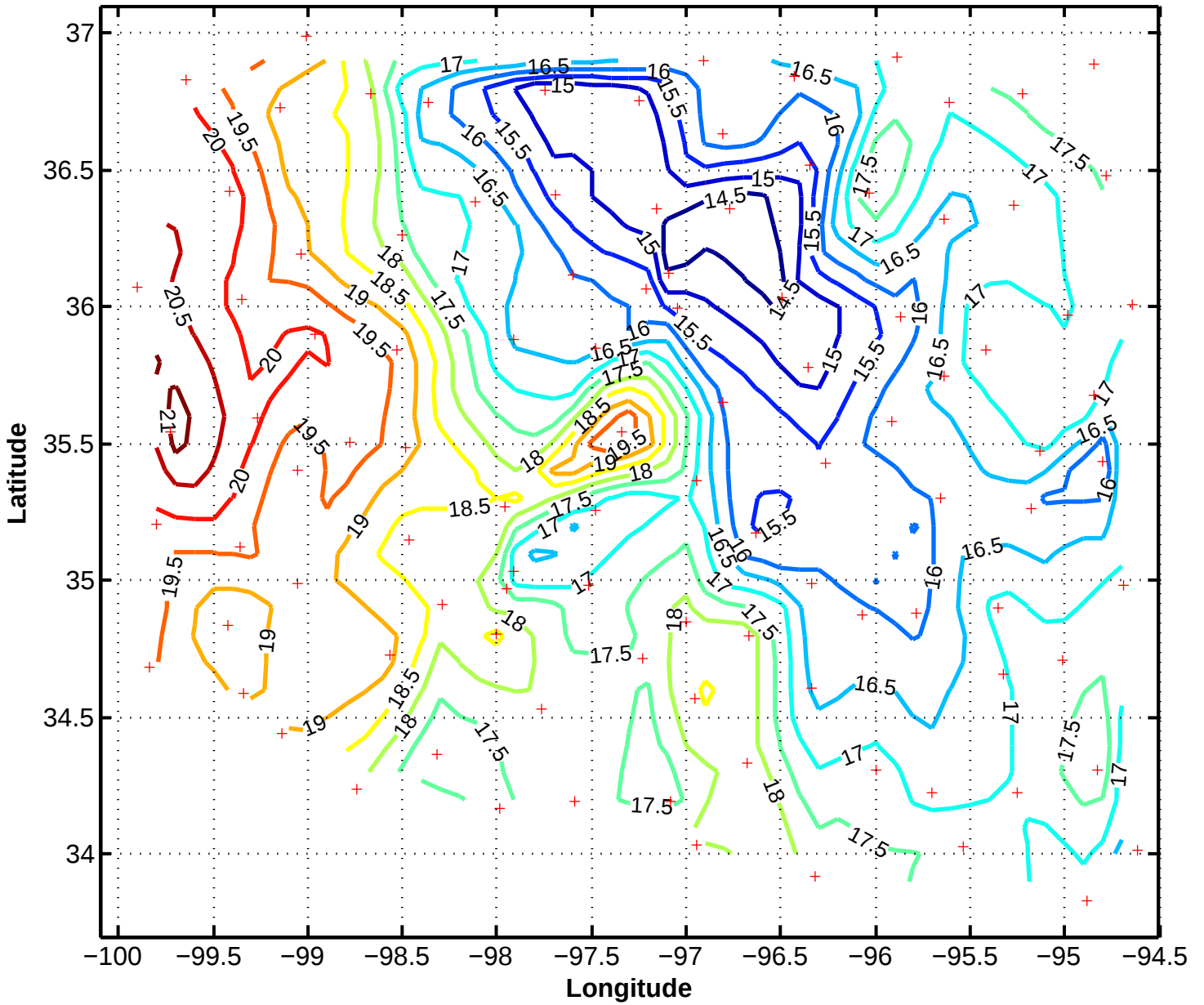
6/11/97 1200z Mesonet Temperature (Celsius)
