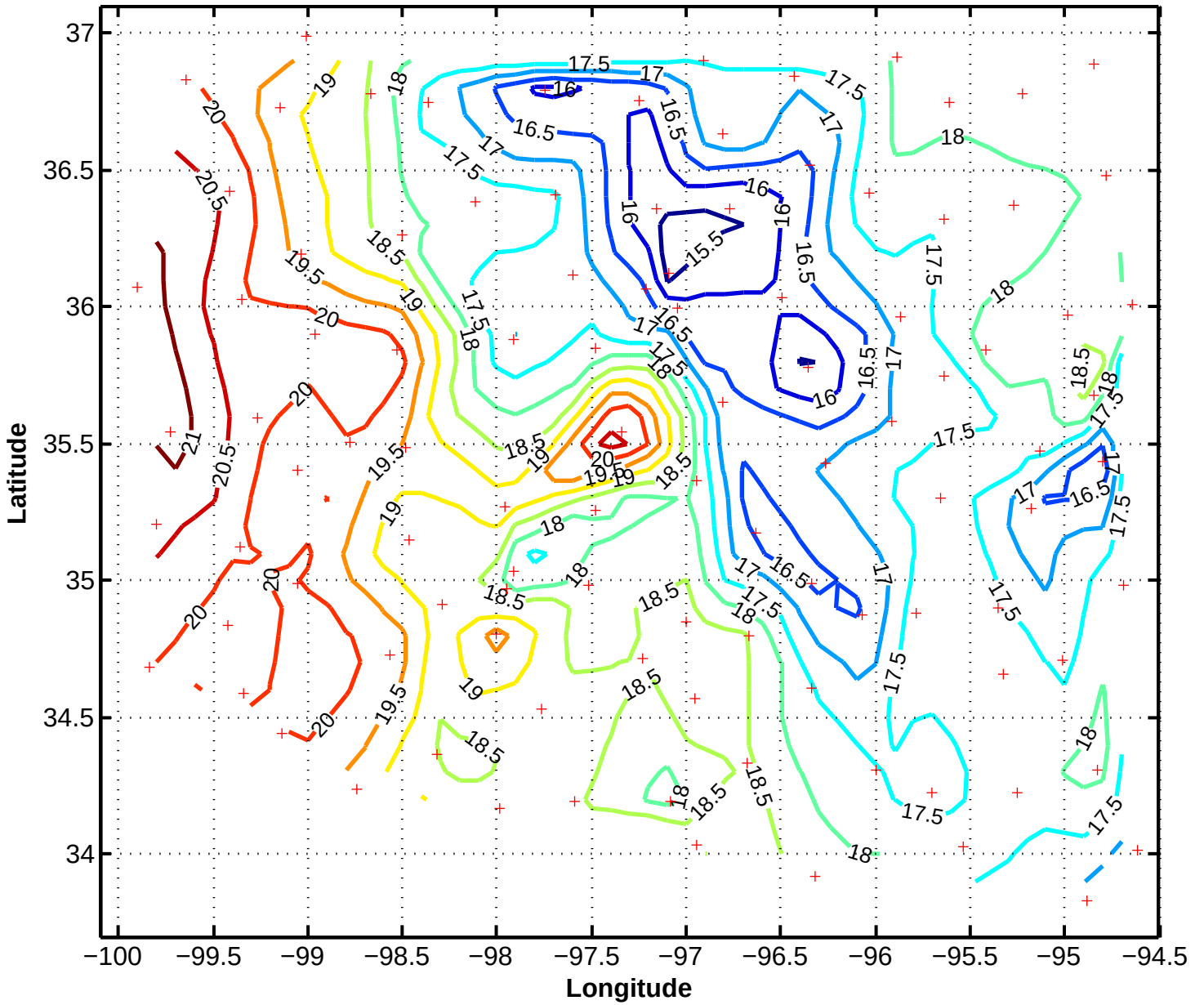
6/11/97 1230z Mesonet Temperature (Celsius)
