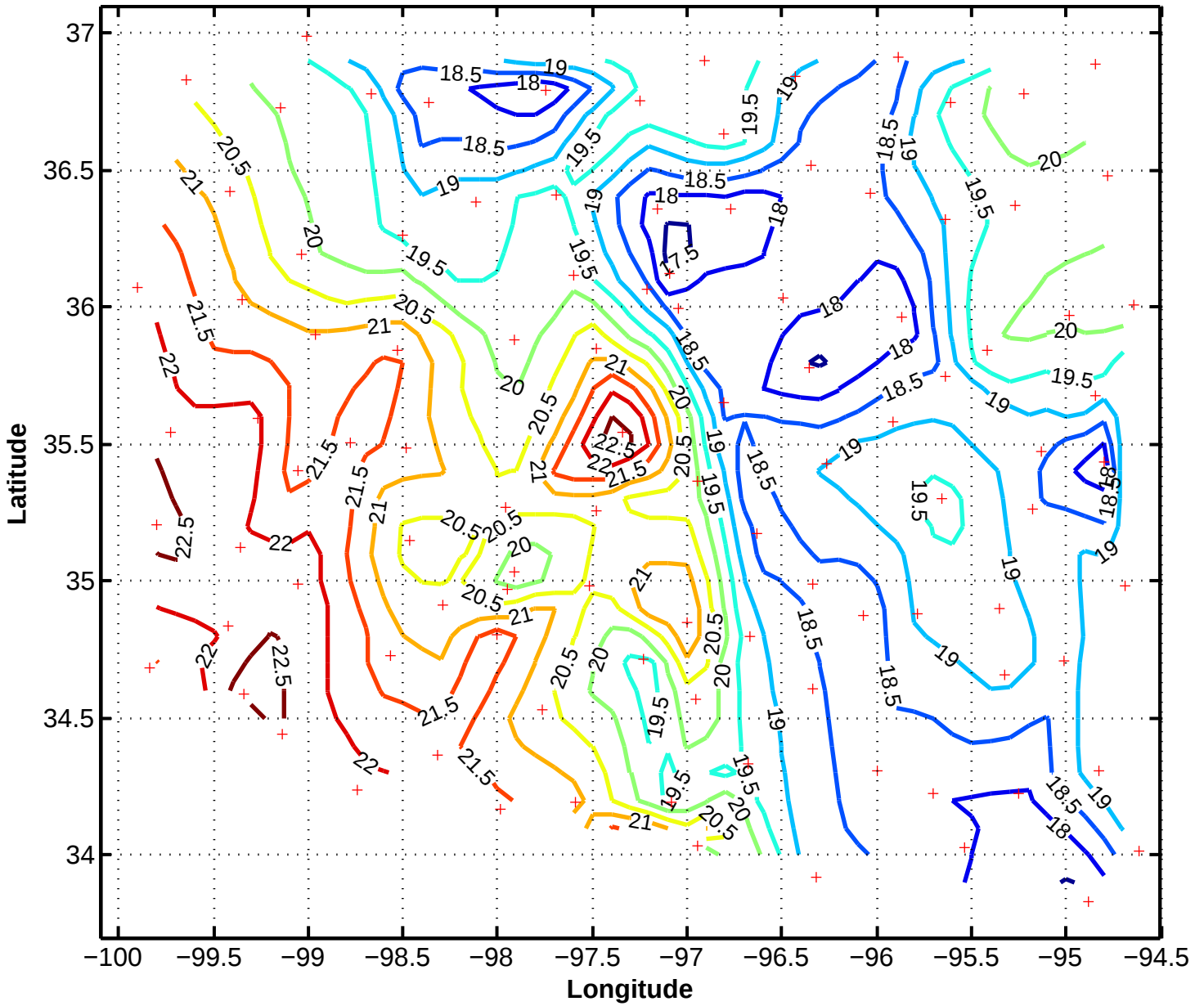
6/11/97 1330z Mesonet Temperature (Celsius)
