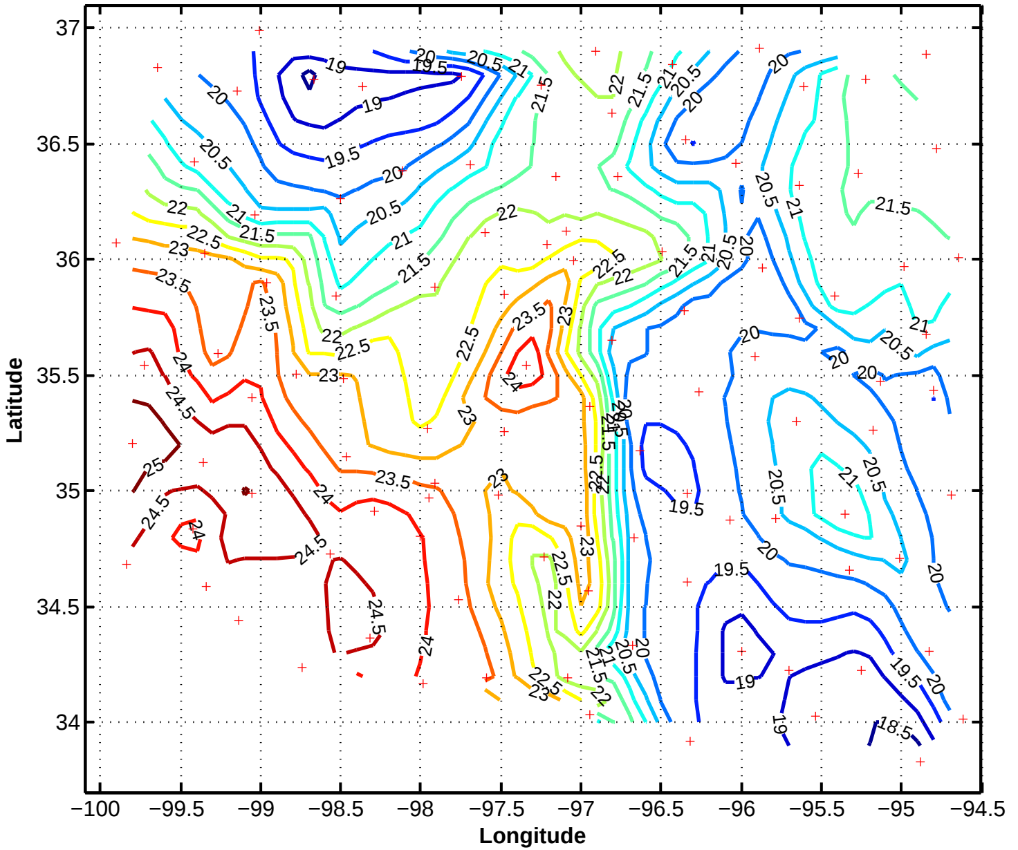
6/11/97 1430z Mesonet Temperature (Celsius)
