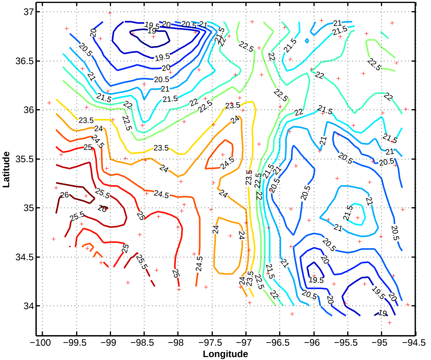
6/11/97 1500z Mesonet Temperature (Celsius)
