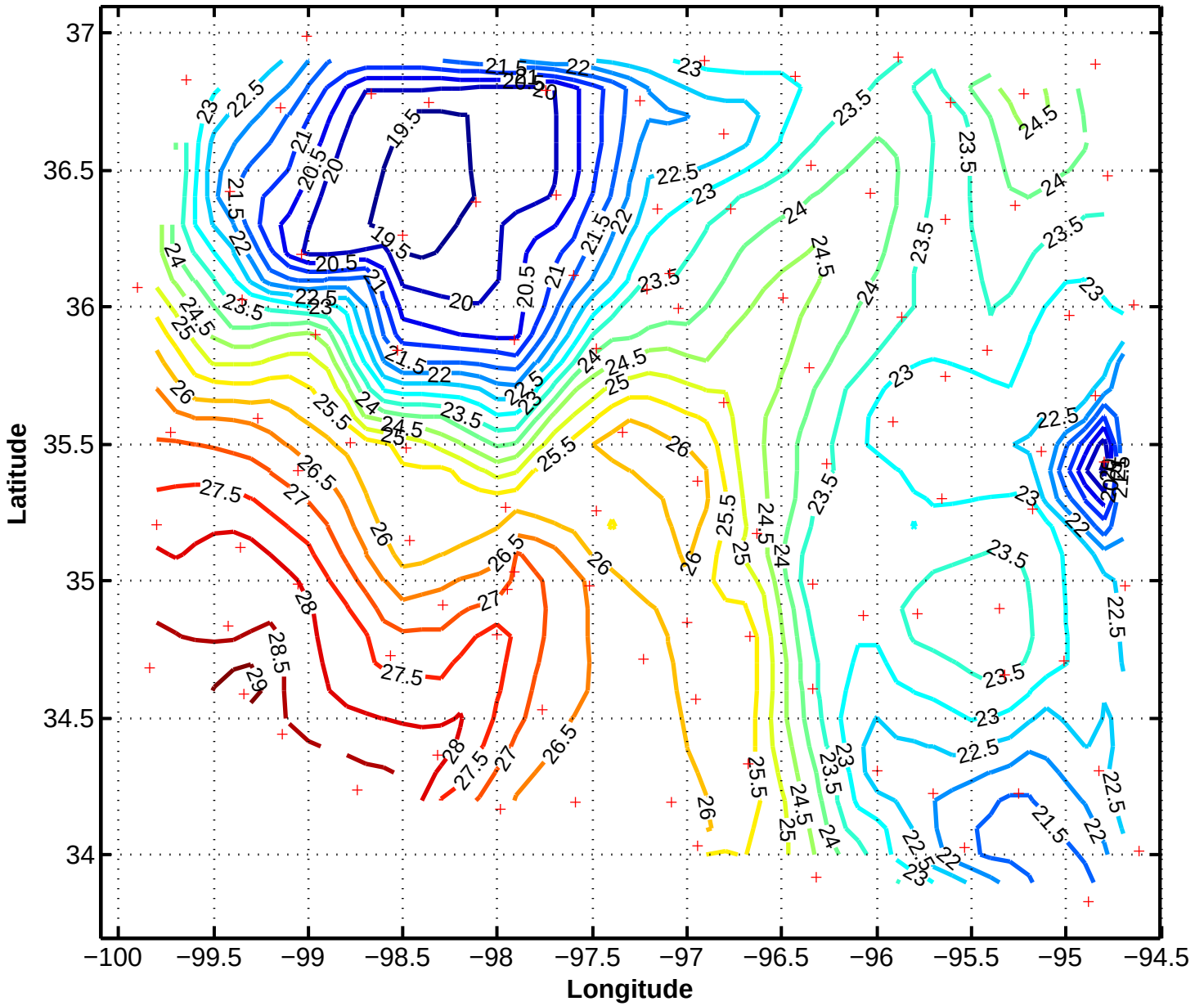
6/11/97 1630z Mesonet Temperature (Celsius)
