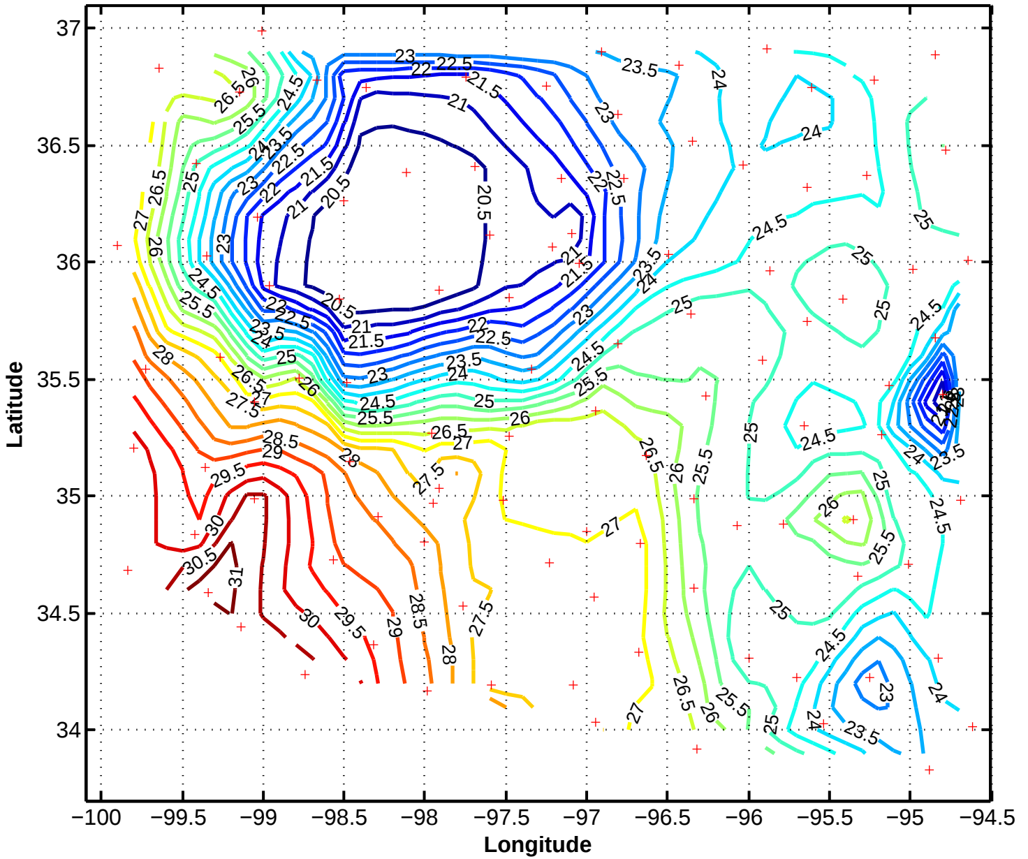
6/11/97 1800z Mesonet Temperature (Celsius)
