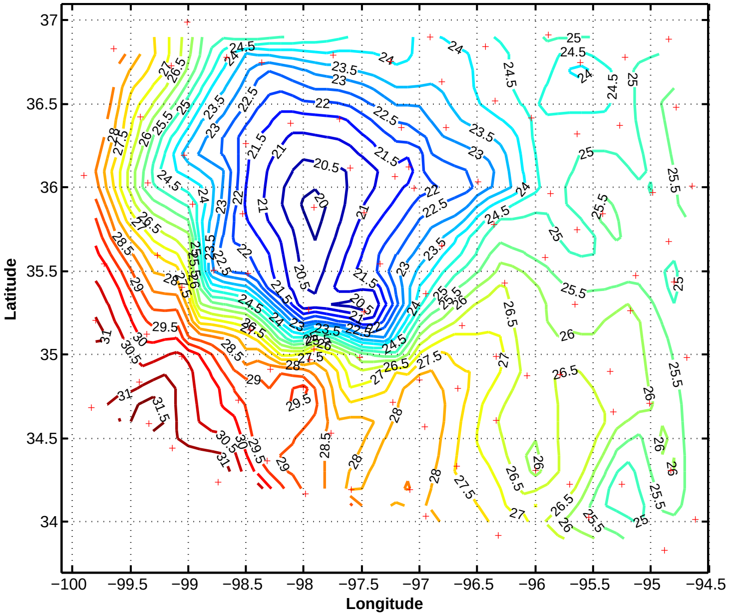
6/11/97 1900z Mesonet Temperature (Celsius)
