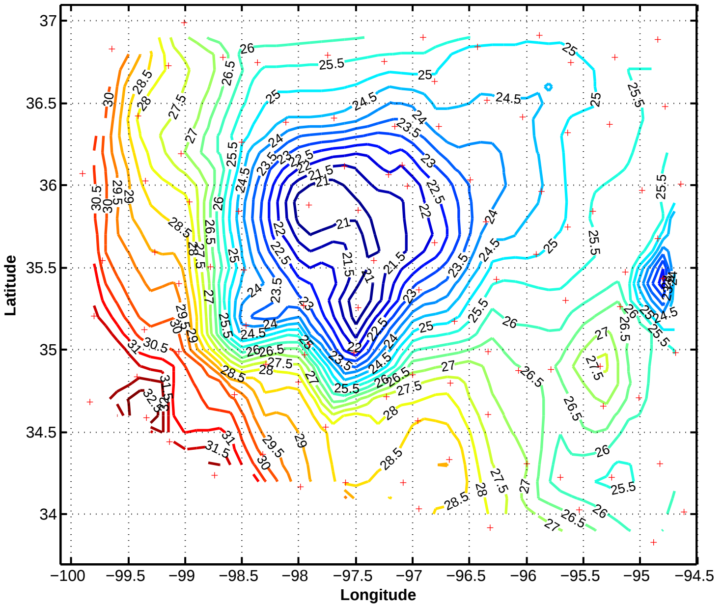
6/11/97 2000z Mesonet Temperature (Celsius)
