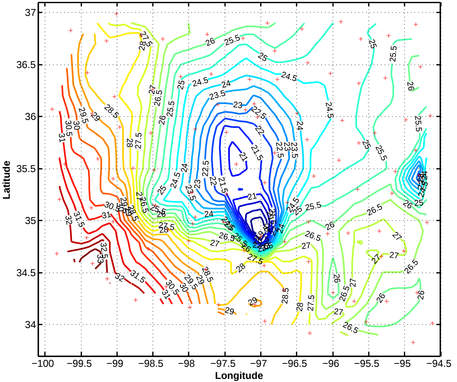
6/11/97 2030z Mesonet Temperature (Celsius)
