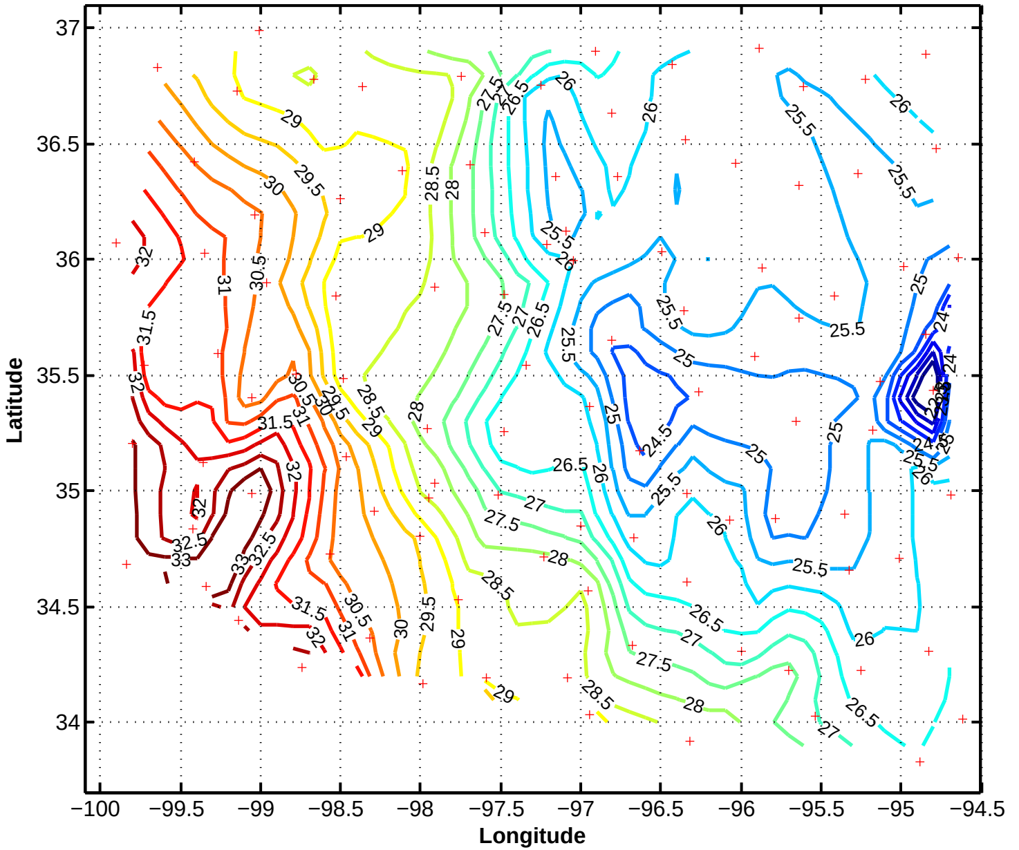
6/11/97 2230z Mesonet Temperature (Celsius)
