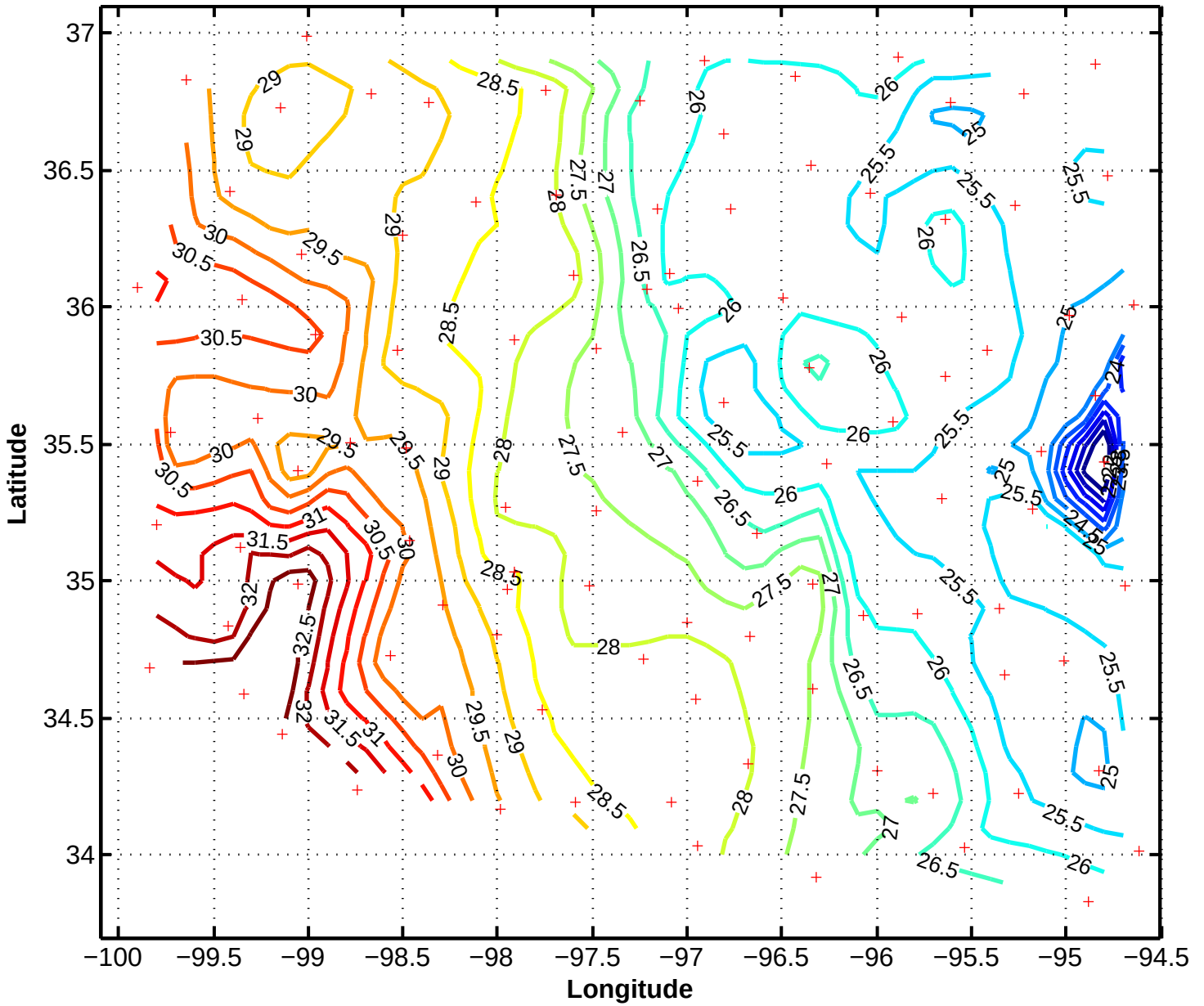
6/11/97 2330z Mesonet Temperature (Celsius)
