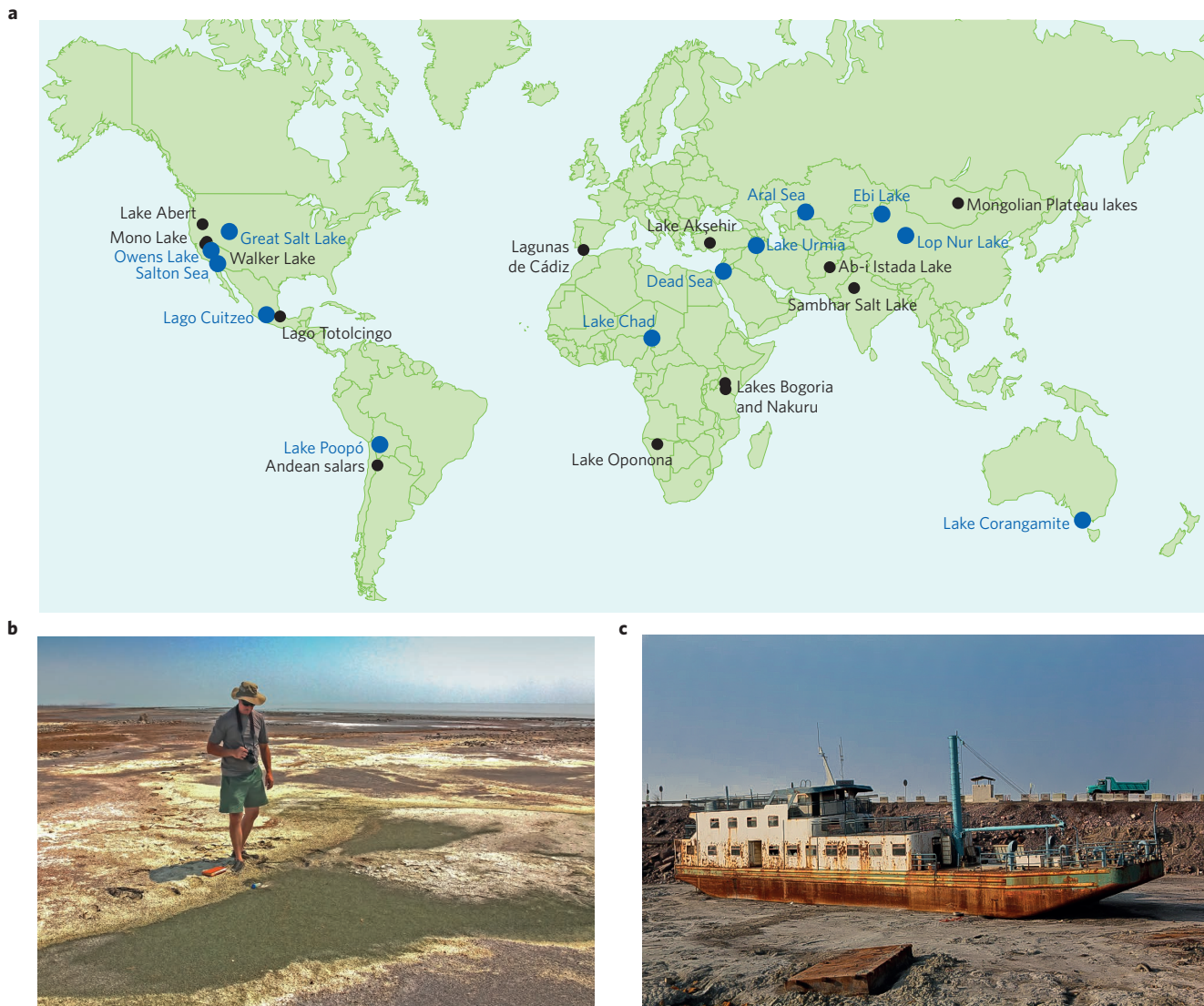
Figure 1 | The world's declining saline lakes. a , Some of the world's salt lakes that have been impaired by water diversions and/or climate change. Larger symbols indicate lakes formerly larger than 250 km 2 . b , A limnologist inspects a pond left behind on the lakebed of the receding Great Salt Lake (USA; August 2012). c , Stranded ship on the dry lakebed of Lake Urmia (Iran; February 2014). Photographs courtesy of W. A. Wurtsbaugh.
