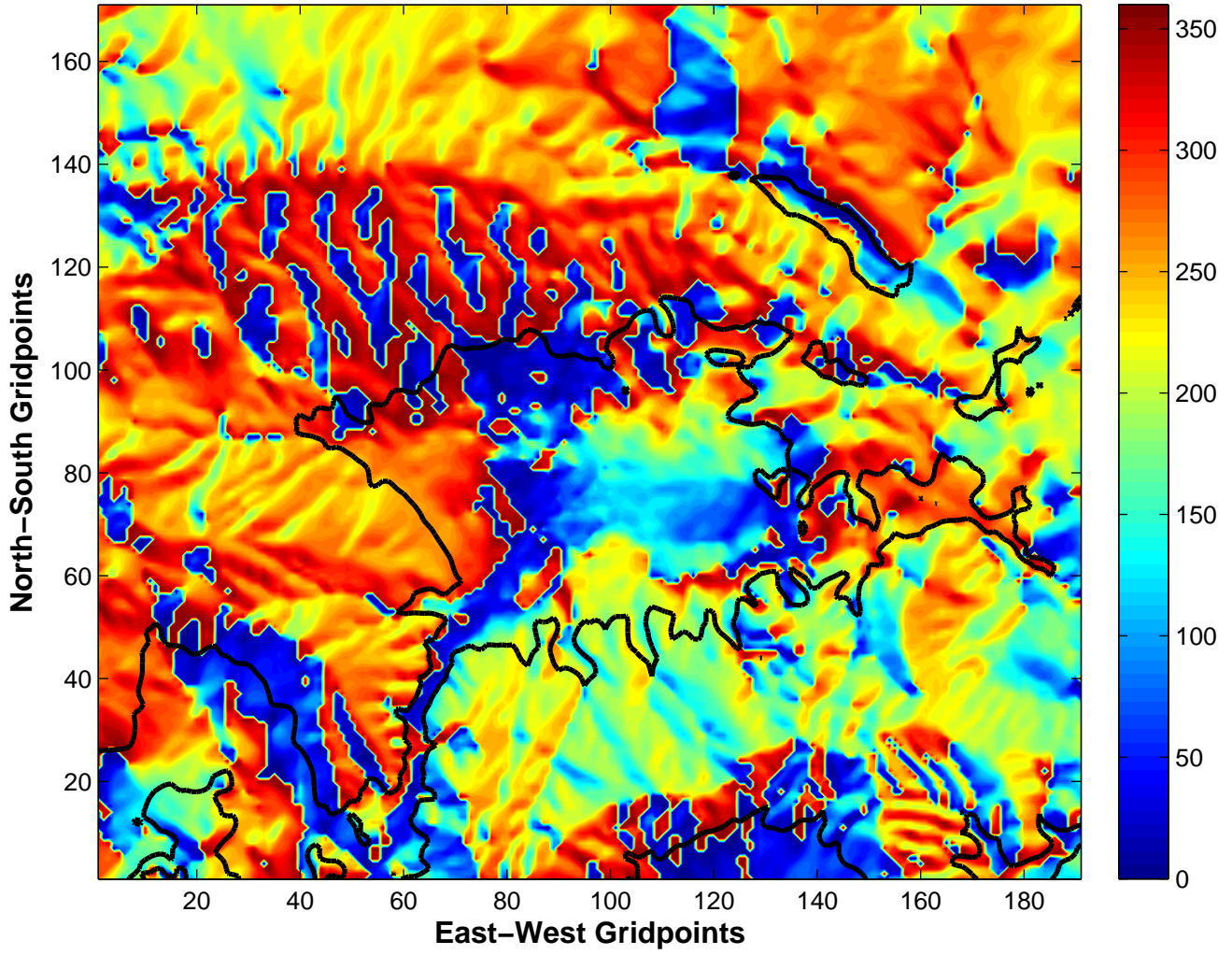
Mean 10-m Wind Direction (degrees) – BASE Average for night hours
