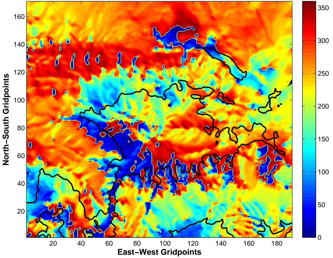
Mean 10-m Wind Direction (degrees) – BASE Average for day hours
