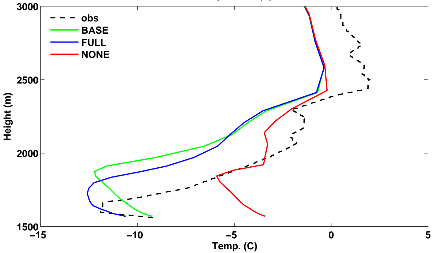
18 UTC 5 Feb 2013 Temperature (C)
