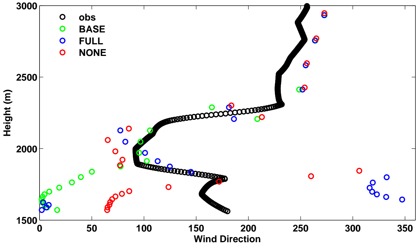
18 UTC 5 Feb 2013 Wind Direction (degrees)
