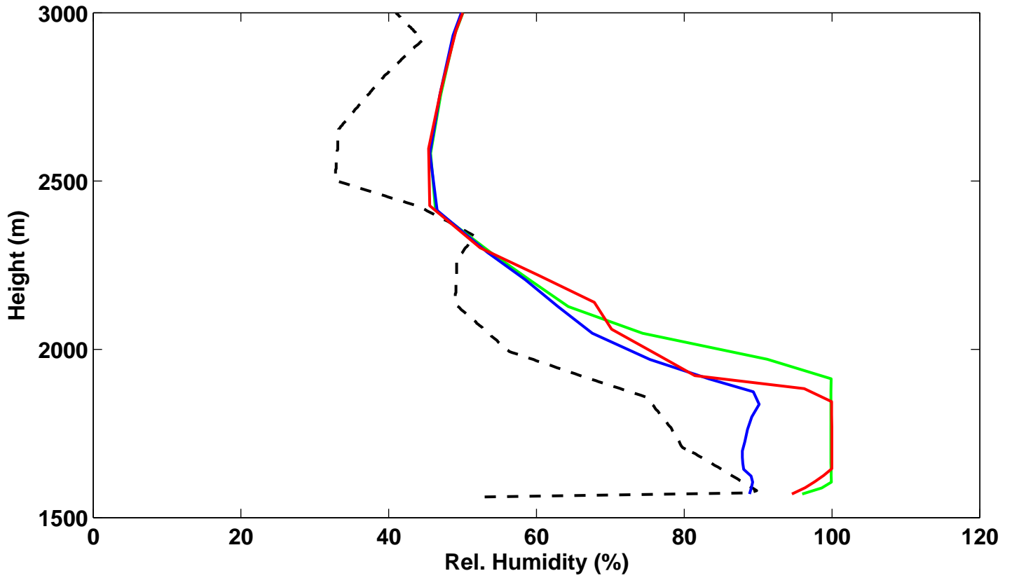
18 UTC 5 Feb 2013 Rel. Humidity wrt Water
