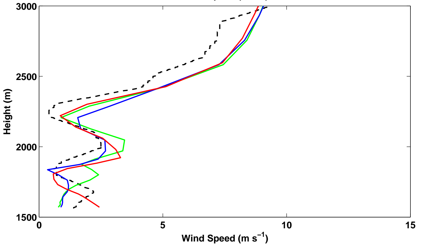
18 UTC 5 Feb 2013 Wind Speed ( \text{m s}^{-1} )
