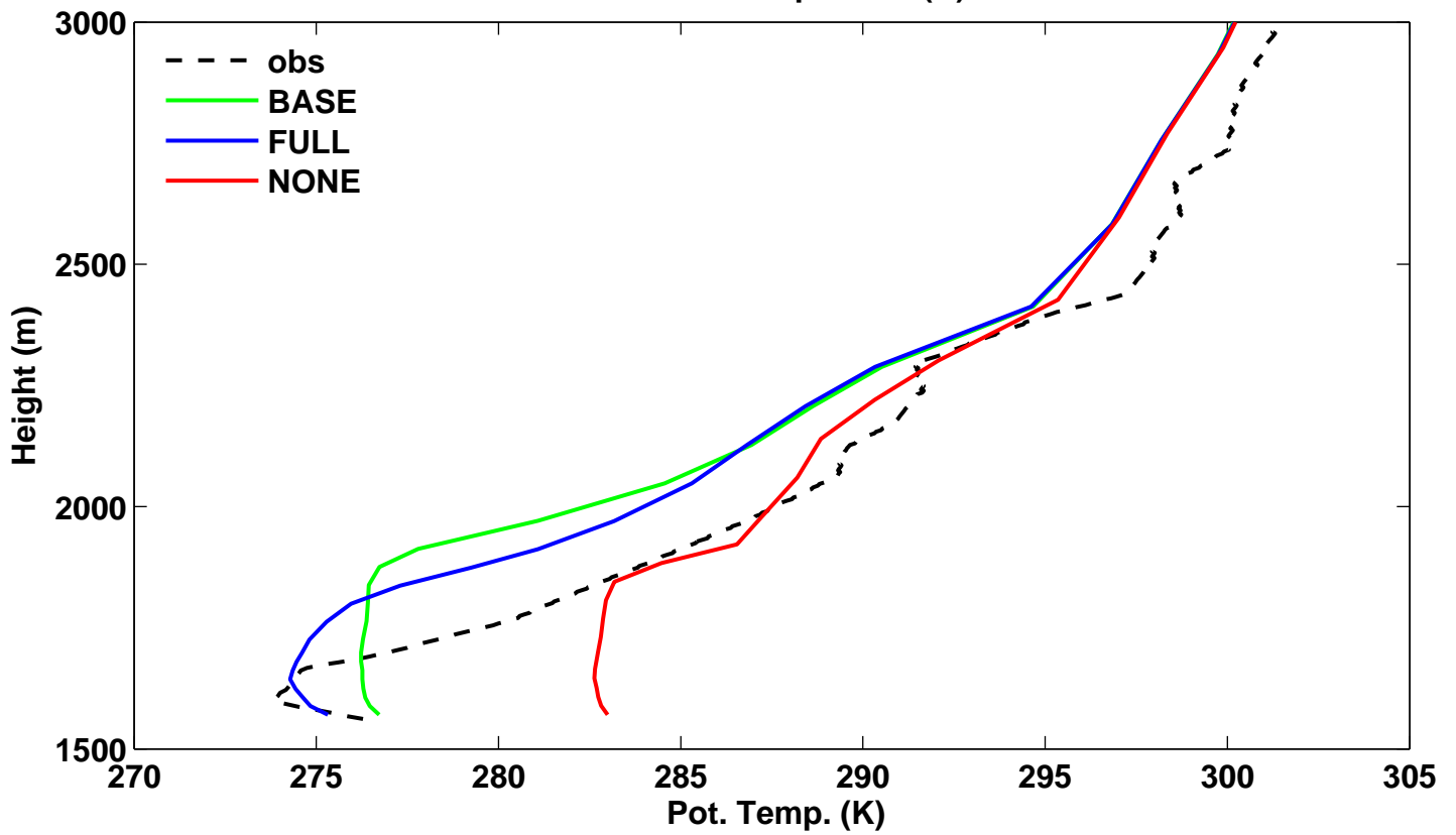
18 UTC 5 Feb 2013 Potential Temperature (K)
