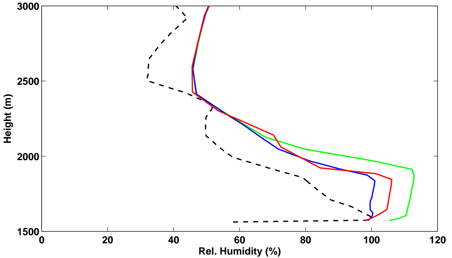
18 UTC 5 Feb 2013 Rel. Humidity wrt Ice
