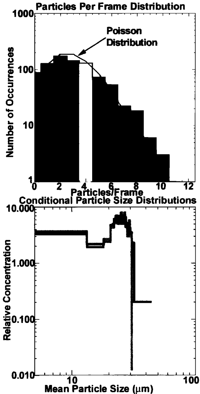
Figure 3. (top) Histograms of the number of particles per frame for all the CPI imaged frames during the time period 2209:45 – 2210:25 shown in Figure 2 along with the Poisson distribution with the same mean, and (bottom) conditional particle size distributions produced by using only those particles in frames with five or more particles (black) and by using those particles in frames with three or fewer particles per frame (grey).
