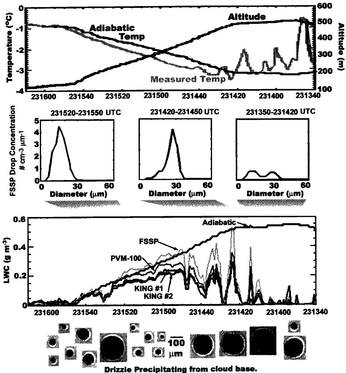
Figure 7. (top) Time series of the temperature and altitude recorded by the C-130 on July 29, 1998, as it sampled a boundary layer cloud and the calculated adiabatic temperature. (middle) FSSP size distributions for different time periods. (bottom) A time series of LWC recorded by several different probes is compared to the calculated adiabatic value.
