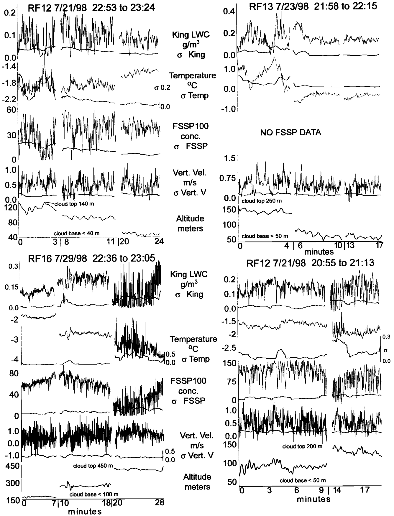
Figure 10. Time series of measurements and their standard deviations made by the C-130 as it flew different level passes through boundary layer clouds on four different occasions.
