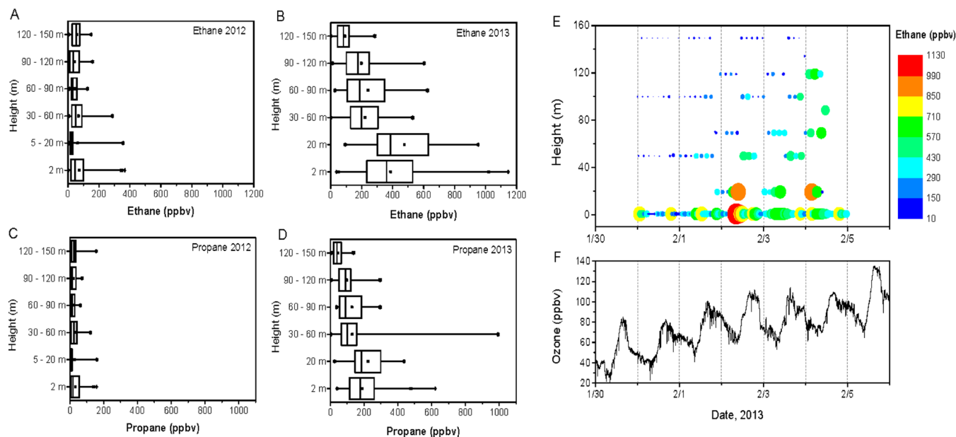
Figure 6. Box-whisker plots showing the vertical distribution of ethane and propane during both experiments (left) from all available tethered balloon data, with the 2-m data filtered for times when the balloon was up. Boxes outline the 25–75 percentile of the data, the vertical line inside the box the median, the dots the mean, and the whiskers the minimum and maximum values. The right panel shows the buildup of ethane with height and time during the Jan 31–Feb 9, 2013, ozone pollution event, with the circle size being proportional to the measured ethane mole fraction, and ozone measured from the 2-m tower inlet.
