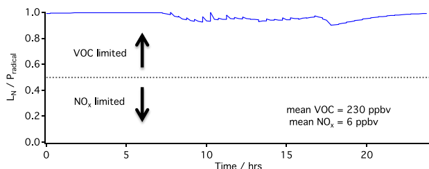
Fig. 12. Calculated L_N/P_{\text{radical}} ratio for the constrained model day.
