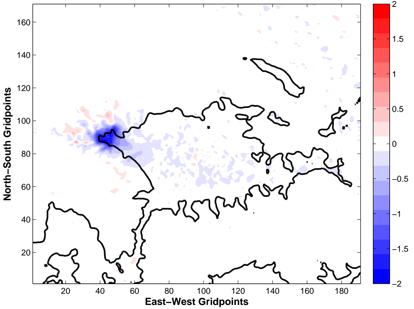
10-m U-wind Difference (m/s) No Wrn Snow - Full Snow Difference Average for all Daytime Hours (15-00 UTC)
