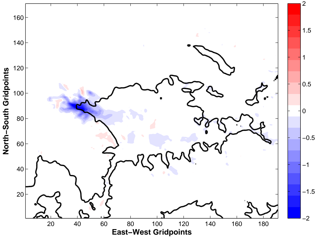
10-m U-wind Difference (m/s) No Wrn Snow - Full Snow Difference Average for all Nighttime Hours (01-14 UTC)
